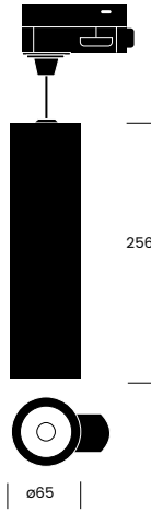
Dimensions in mm
